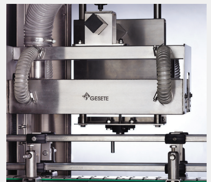
Specially designed bottle cap/neck drying device.
